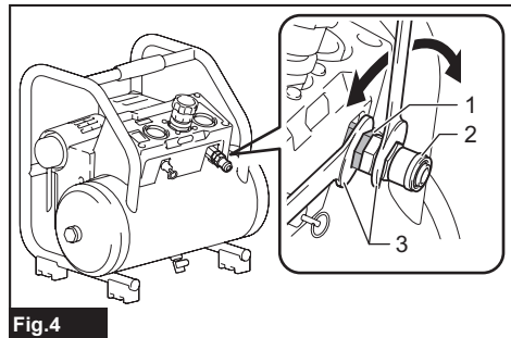
► 1. Air outlet 2. Quick coupler 3. Wrench
